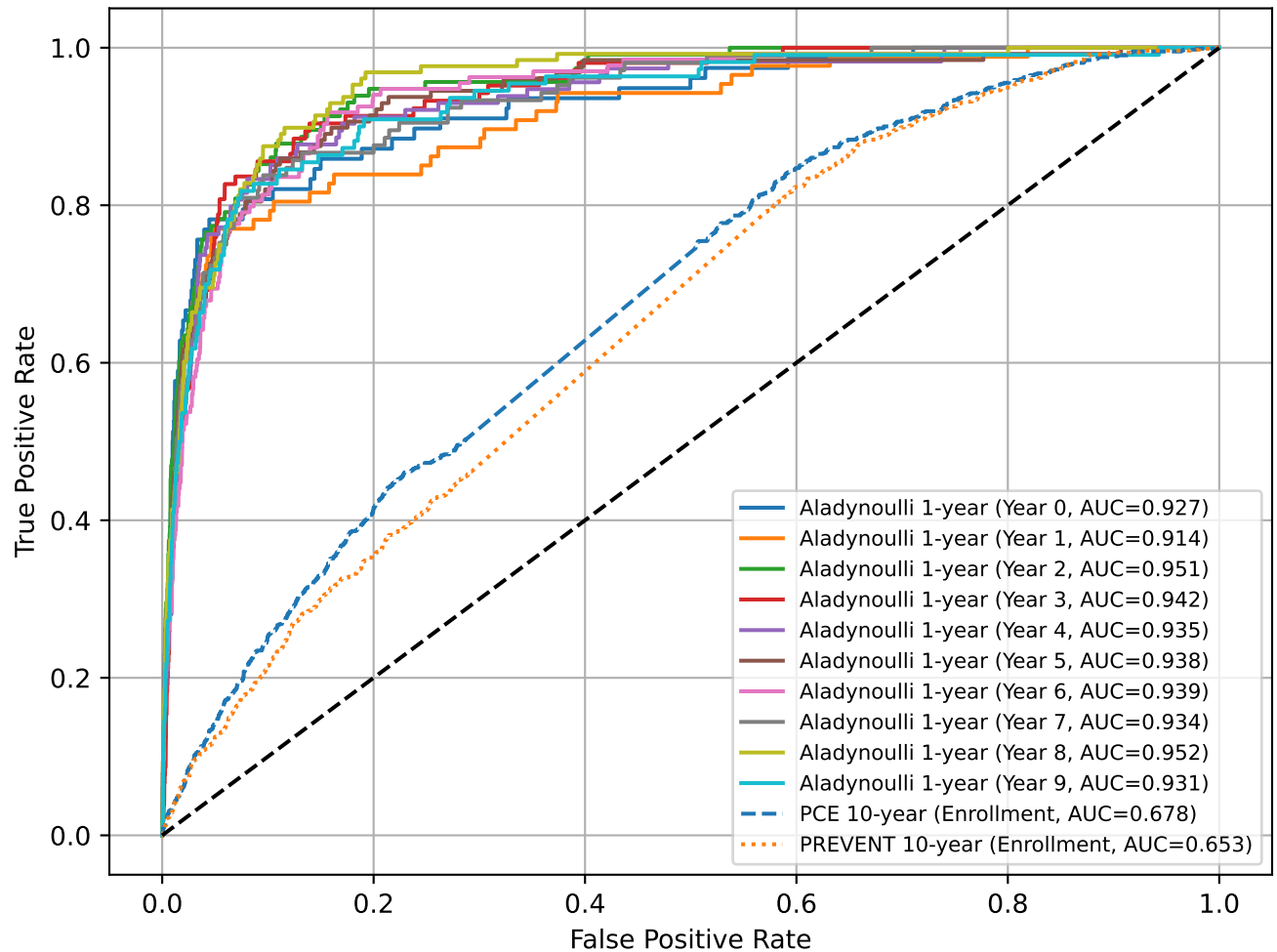
ROC Curves for ASCVD (Reparam): Aladynoulli 1-year (All Offsets) vs PCE/PREVENT 10-year
